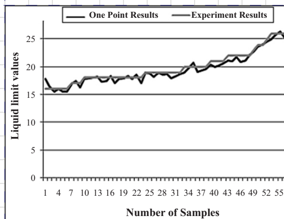
Fig. 6. Comparison of LL b/w One Point & Experimental Results @ 20 number of Blows
